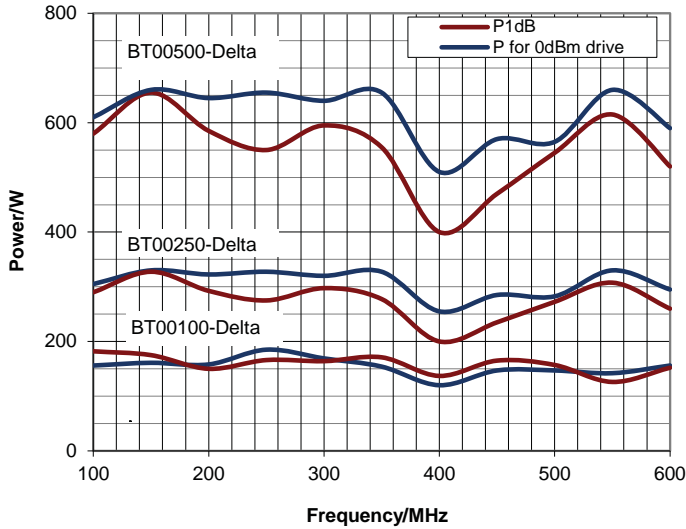
Typical peak envelope power plots
