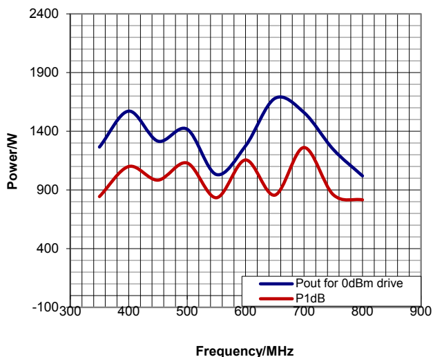
Typical peak output power plots
