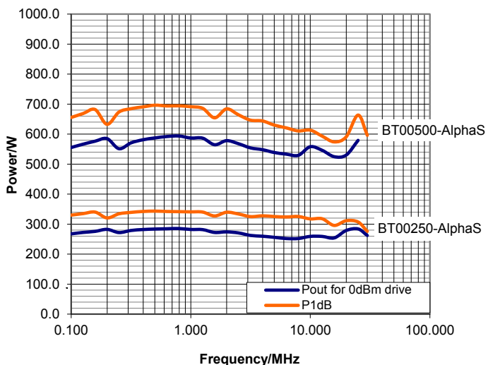
Typical peak output power plots
