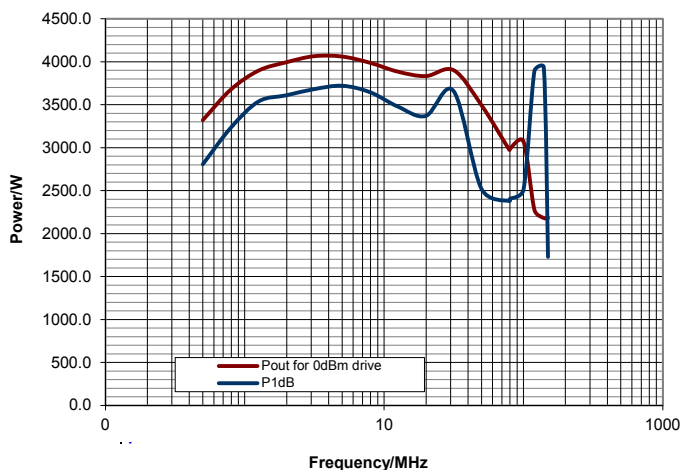
Typical peak envelope power plots
