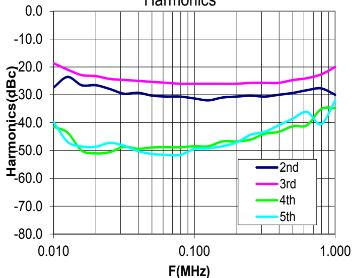
Harmonics
