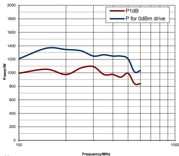
Typical peak envelope power plots
