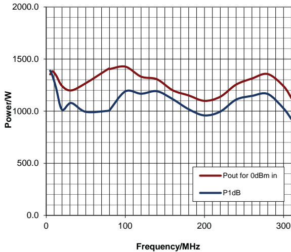
Typical peak envelope power plots
